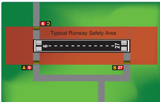
Figure 14-7. Runway Safety Area.
