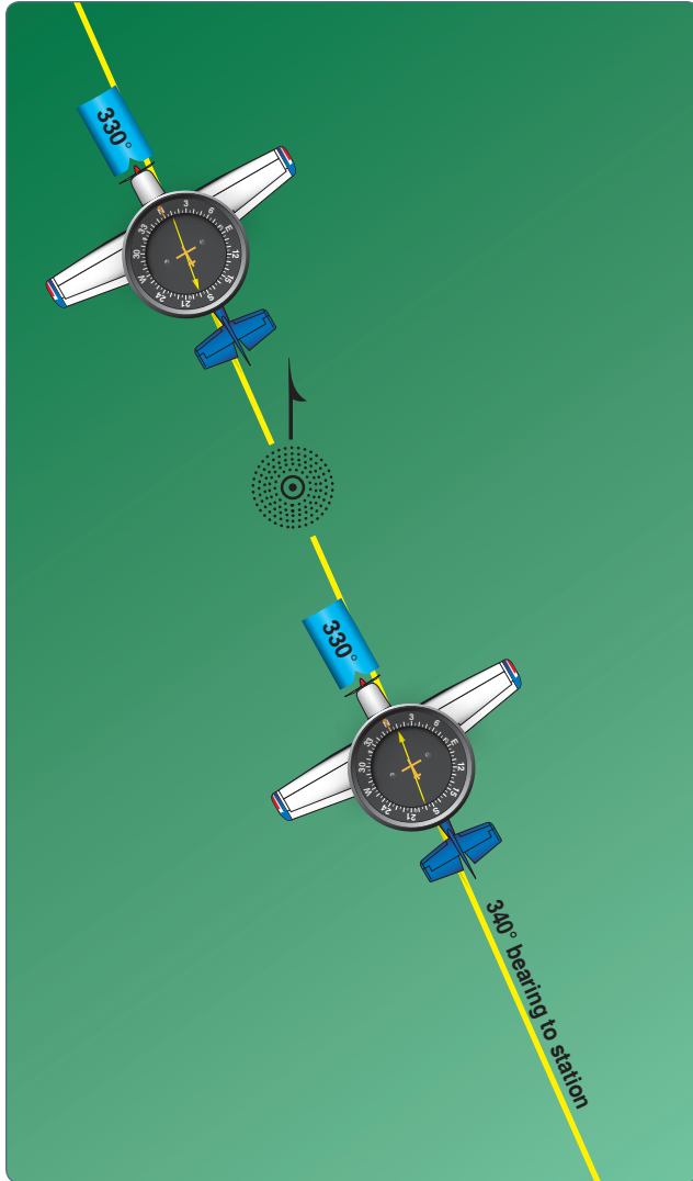
Figure 16-39. ADF tracking.
