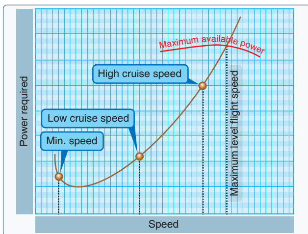
Figure 11-6. Power versus speed.
