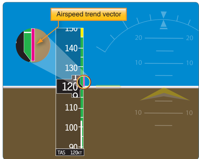
Figure 8-16. Airspeed trend vector.
