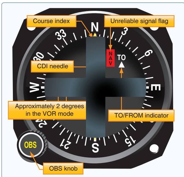
Figure 16-29. VOR indicator.
