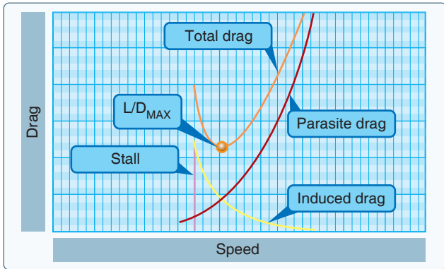
Figure 11-5. Drag versus speed.
