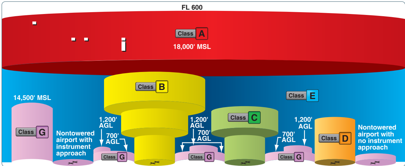
Figure 15-1. Airspace profile.
